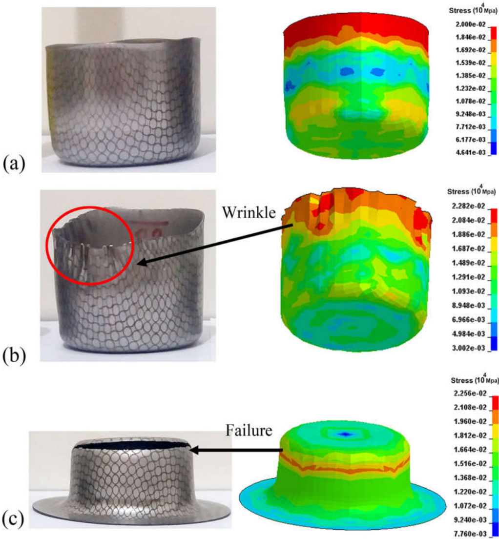
Fig. 5. Stress concentration, wrinkle and failure area of the drawn cup from a blank diameter of 80 mm under (a) optimum, (b) low and (c) high blank holder forces condition
