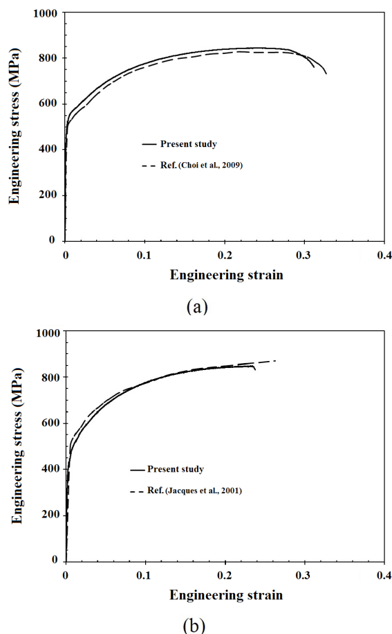
Fig. 4. Uniaxial engineering stress-strain curves of the studied materials together with those which reported for steels with similar microstructure and chemical composition: (a) TRIP1 (b) TRIP2.
