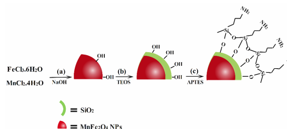
Fig. 2. Schematic illustration of \text{MnFe}_2\text{O}_4@ \text{SiO}_2\text{-NH}_2 nanocomposite particles preparation: (a) synthesis of \text{MnFe}_2\text{O}_4 NPs, (b) formation of \text{SiO}_2 shell, and (c) synthesis of \text{MnFe}_2\text{O}_4@ \text{SiO}_2\text{-NH}_2 NPs
