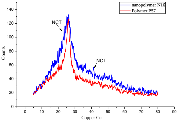
Fig. 9. X-ray diffraction (XRD) curve of poly 2-Aminobenzothiozol (red curve), poly 2-aminobenzothiozol: MWCNTs composite
