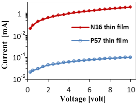
Fig. 10. Current-Voltage (I-V) characteristics of the pure polymer (P57) and 2-aminobenzothiozole: MWCNTs composite (N16) thin films under dark conditions
