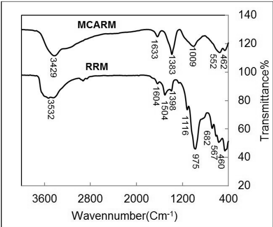
Fig. 2. FTIR spectra of RRM and MCARM.
