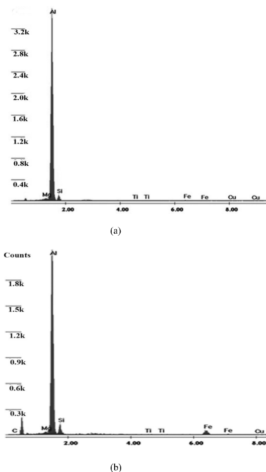
Fig. 16. EDS analysis of worn out surfaces (a) base alloy and (b) composite
