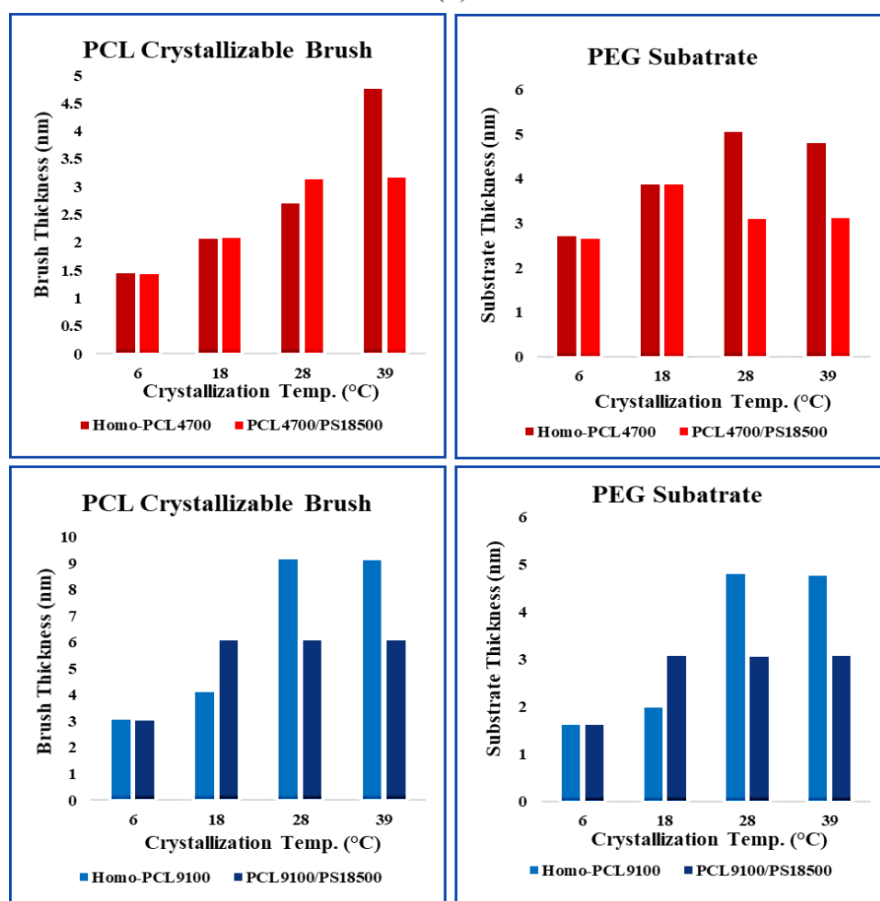
Fig. 3. AFM height images and the corresponding SAED patterns (a) as well as AFM height profiles (b) of PEG 5000 - b -PS 18500 /PEG 5000 - b -PCL 9100 single crystals grown at T c = 6°C (top) and T c = 39°C (bottom), in which the PCL brushes are amorphous and crystalline, respectively; the thickness trends of PCL brushes and PEG substrate via altering the crystallization temperature in PEG 5000 - b -PCL and PEG 5000 - b -PS 18500 /PEG 5000 - b -PCL single crystals (c).
